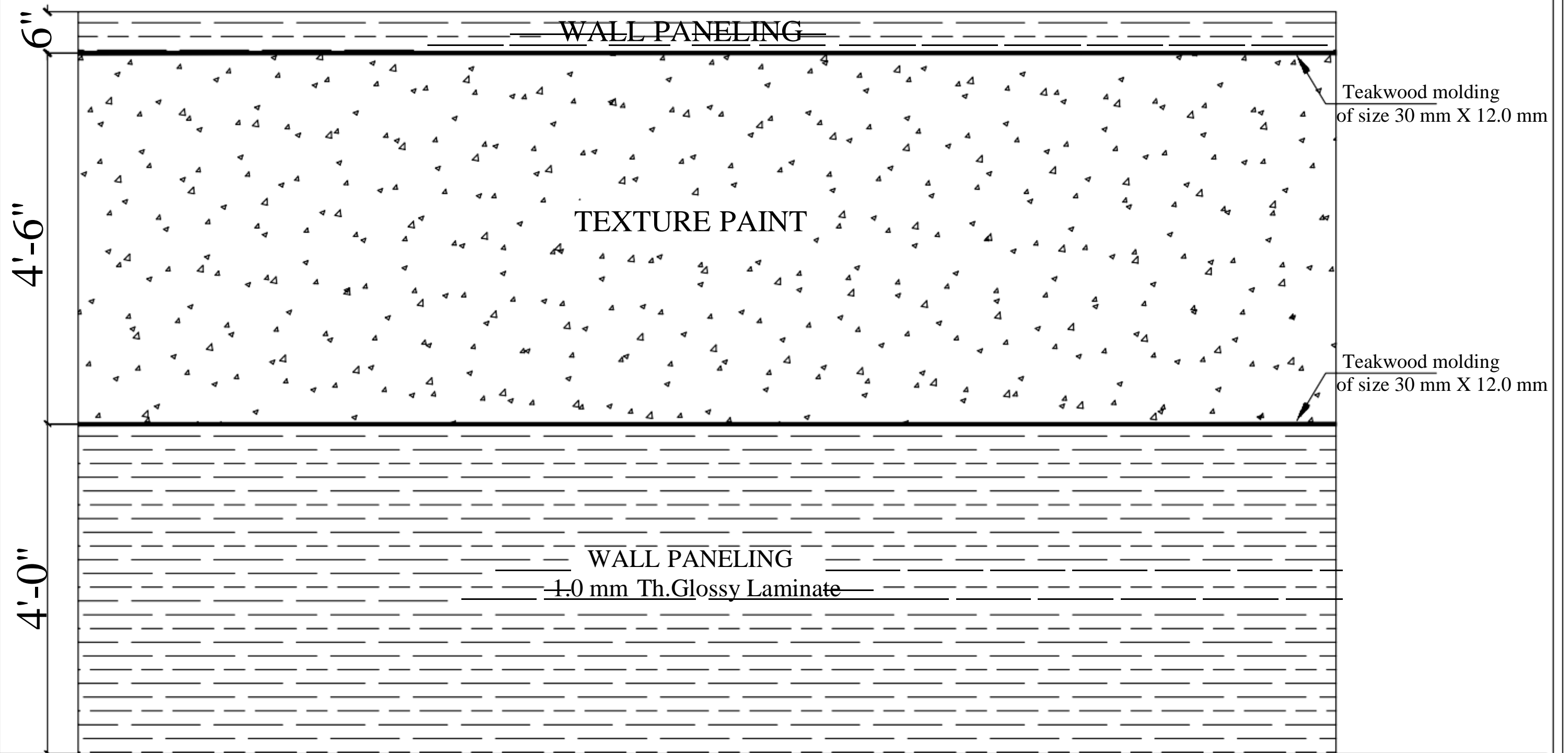
WALL PANELING DETAIL
