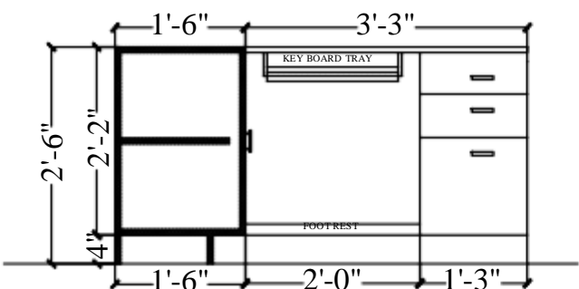
SECTIONAL A-A'
