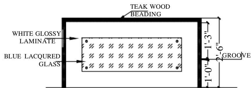
FRONT ELEVATION "Z"
