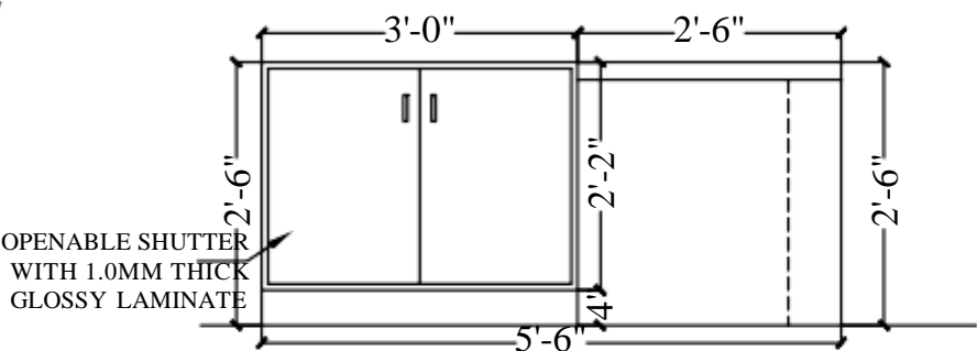
SIDE ELEVATION - X
